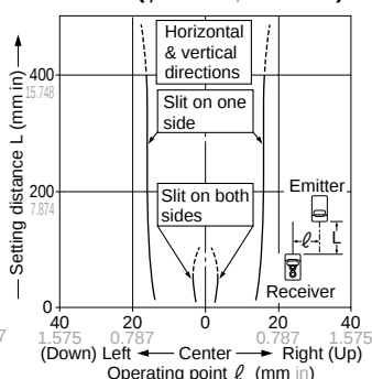
Parallel deviation with rectangular slit masks ( 2 \times 6 mm 0.079 \times 0.236 in)
