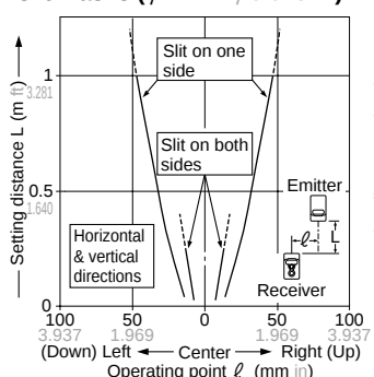
Parallel deviation with round slit masks ( \phi 2 mm \phi 0.079 in)
